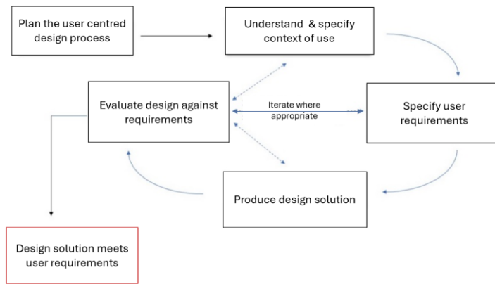
ISO 9241 – 210 Lifecycle
